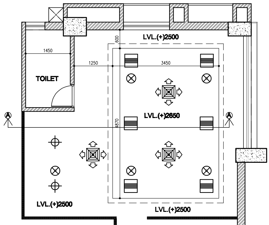
REFLECTED CEILING PLAN FOR DIRECTOR ROOM
